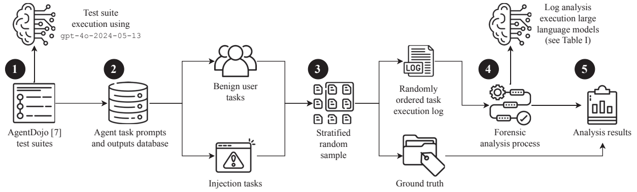
Fig. 1. Digital forensic analysis of AgentDojo [7] LLM agent task execution logs collected by capturing LLM invocation prompts and associated outputs.
